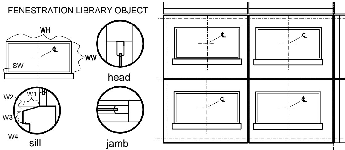
Figure Five – A fenestration library is defined for a project. It includes the panel features that are located with the opening.
