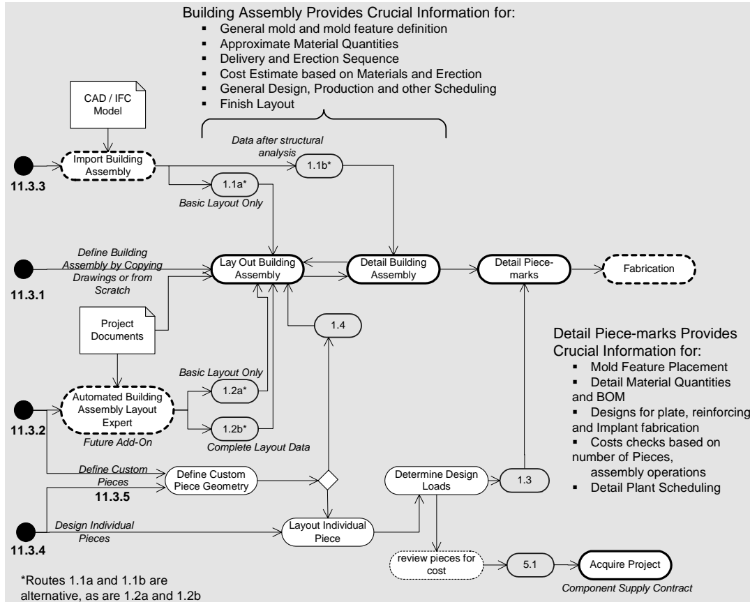
Figure One – A high-level process plan of the functional role of the precast concrete design and engineering application described in this article.
