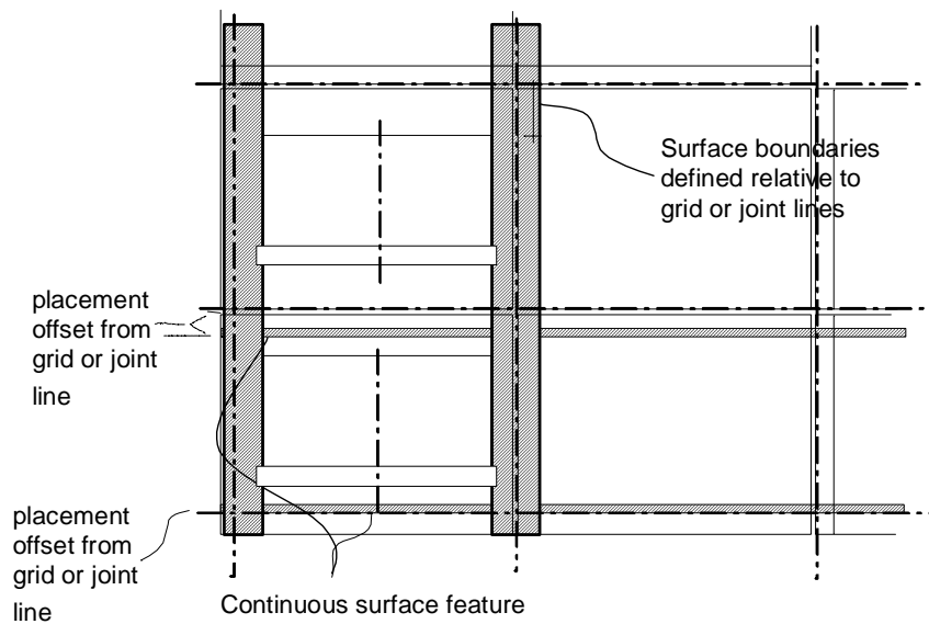
Figure Six – Surface treatment layout is defined parametrically, so that it can be easily adjusted.
